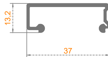
OVAL İÇ RAY
