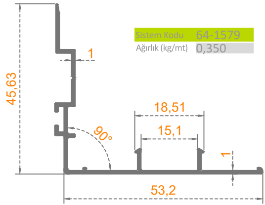
EUROLİNE KENET ( AHŞAP )
