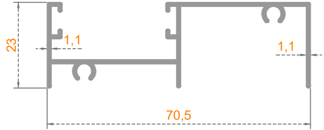
KASA YAN
