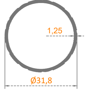
Ø 31.8'LUK BORU
