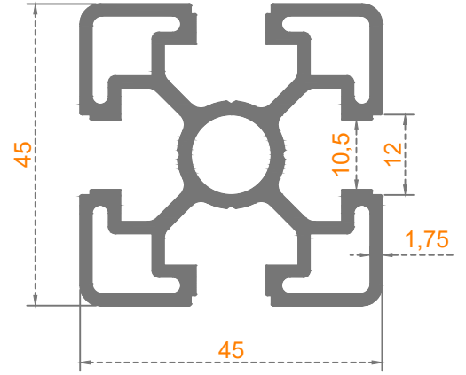
45 x 45 SİGMA PROFİL
