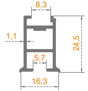
ARKA SABİT
