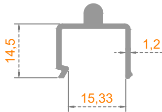
ALT-RAY
