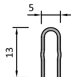
ACC-03 ÇELİK RAY STEEL RAIL
