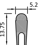
ALÜMİNYUM RAY ALUMINIUM RAIL
